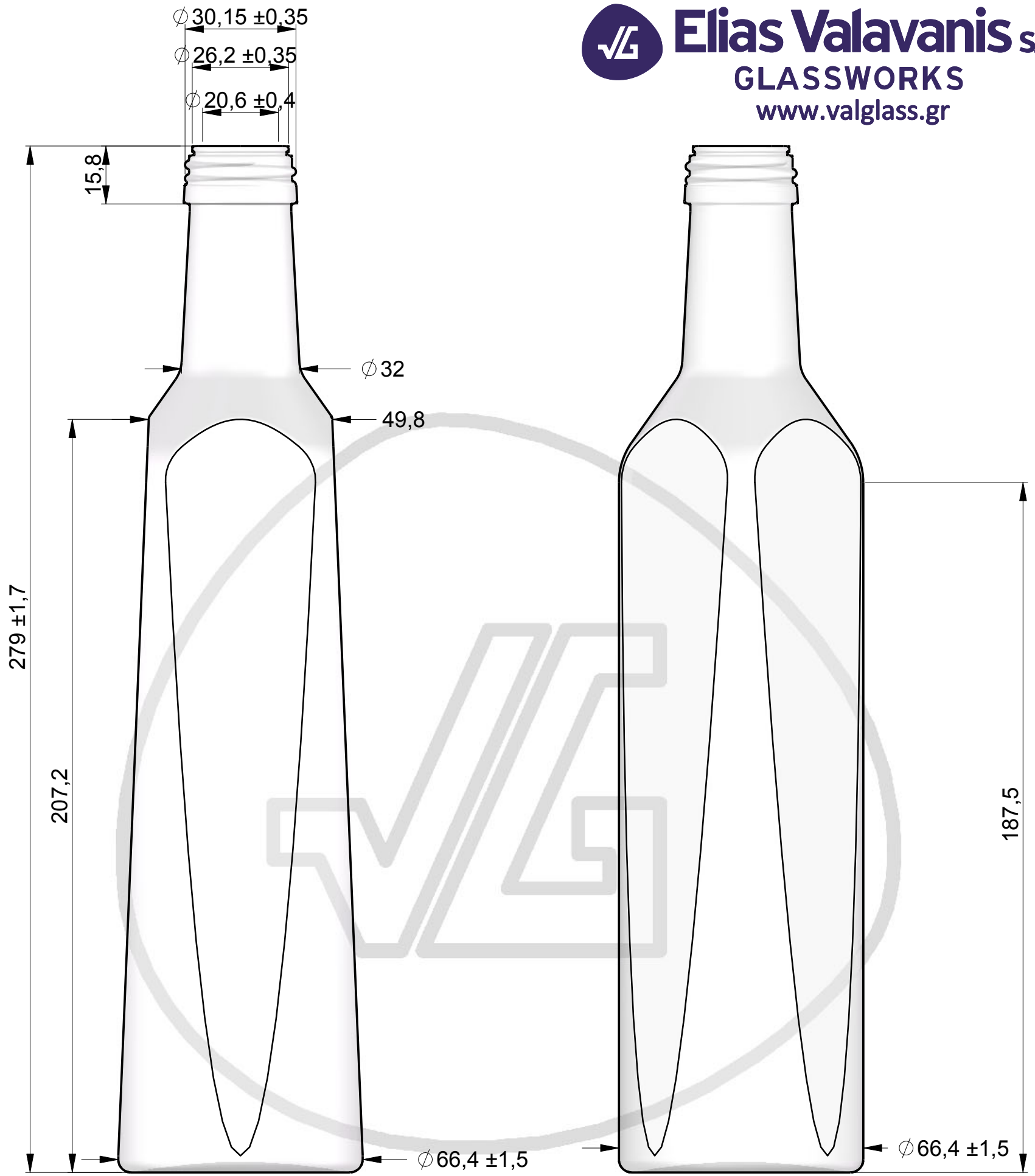
FRONT VIEW
